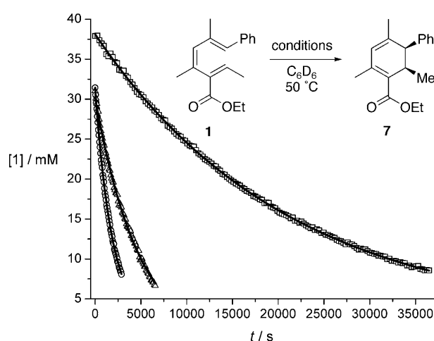
Figure 2. Kinetic plots (with first order exponential decay fits) and half-lives of the electrocycloization of 1 at 50 °C in the presence and absence of Me 2 AlCl. ○: 1 equiv Me 2 AlCl, t 1/2 = 21 min; △: 0.43 equiv Me 2 AlCl, t 1/2 = 41 min; □: thermal, t 1/2 = 4 h.
